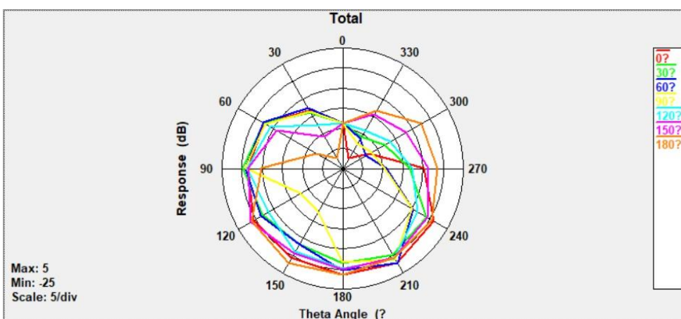
Total @2500 MHz
