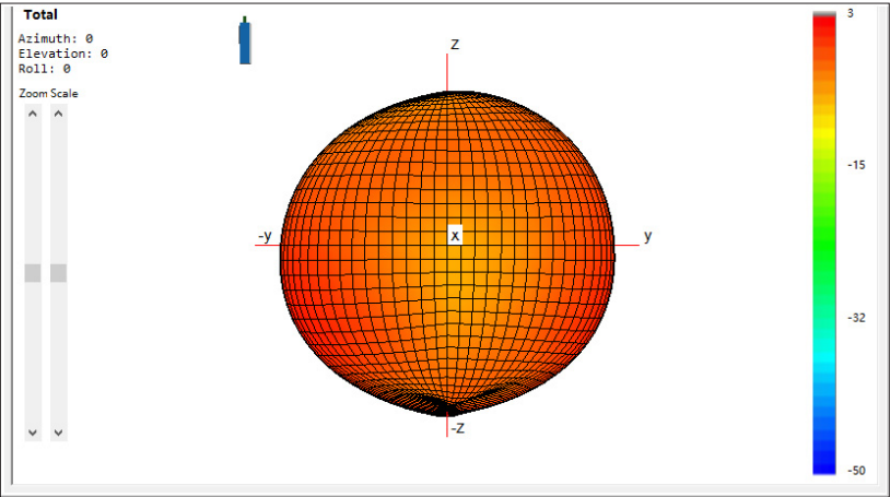
ANT 2 3D radiation patterns @ 2450 MHz
