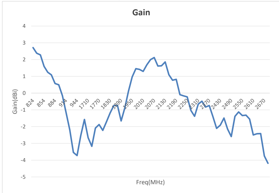
Peak Gain (dBi/Installed on metal surfaces)
