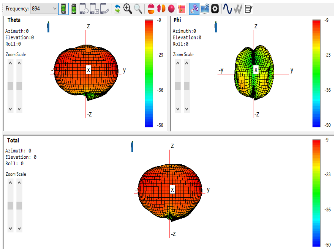
3D Radiation Pattern at 894MHz (Installed on metal surfaces)
