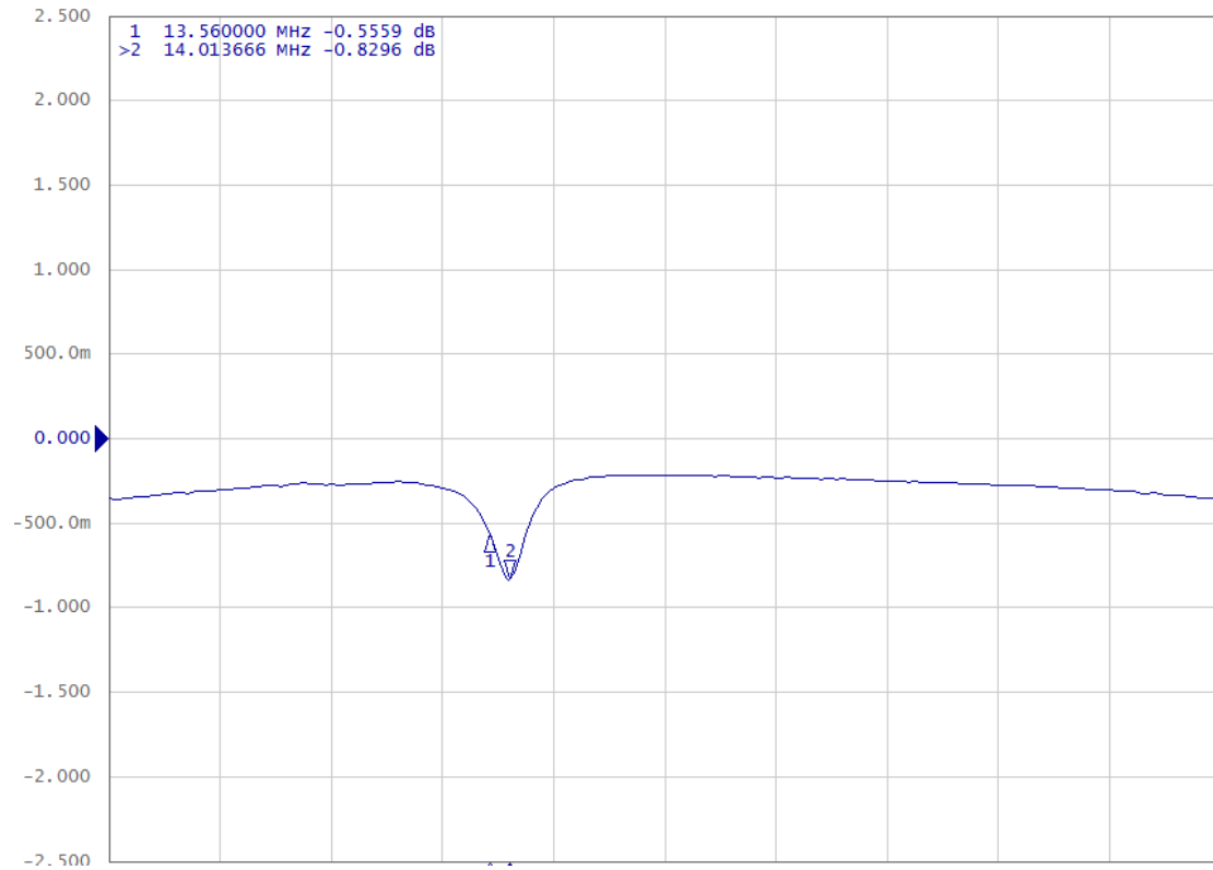
Return Loss
